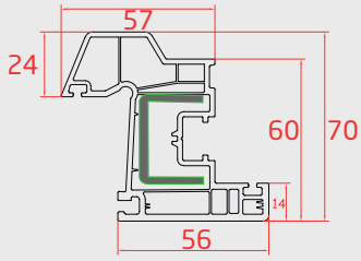
DAMLALIKLI KANAT (Self Drainage Sash Profile)
