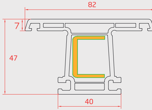
ORTA KAYIT ( Mullion Profile )
