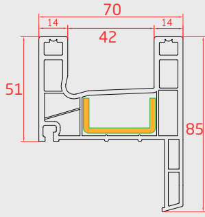
SÜRME PERVAZLI KASA ( Case Profile With Frame )
