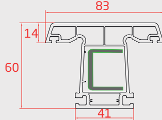
ORTA KAYIT (Mullion Profile)
