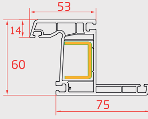
PERVAZLI KASA (Case Profile With Frame)
