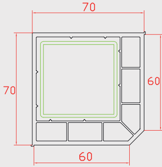
60 - 70 KUTU ( Rectangle Profile )
