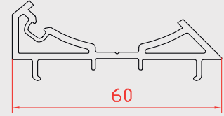
60 mm BORU ADAPTÖRÜ ( Corner Adapter )
