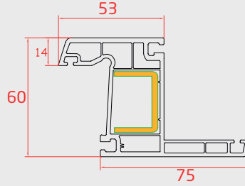
PERVAZLI KASA (Case Profile With Frame)
