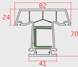
ORTA KAYIT (Mullion Profile)
