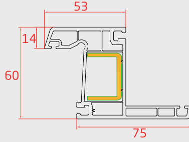
PERVAZLI KASA (Case Profile With Frame)
