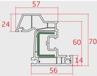
DAMLALIKLI KANAT (Self Drainage Sash Profile)
