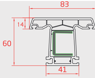
ORTA KAYIT (Mullion Profile)
