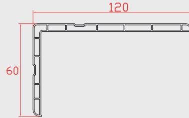
60x120 mm PERVAZ ( Sill Joint Extension Profile )
