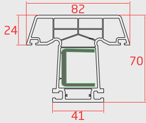
ORTA KAYIT (Mullion Profile)
