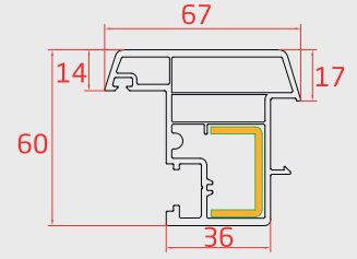
HARAKETLİ ORTA KAYIT (Overhung Profile)
