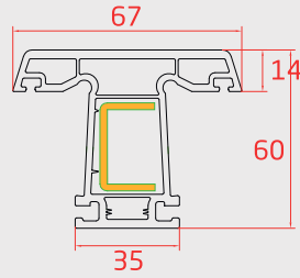
DAR ORTA KAYIT (Mullion Profile)
