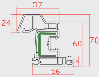
DAMLALIKLI KANAT (Self Drainage Sash Profile)
