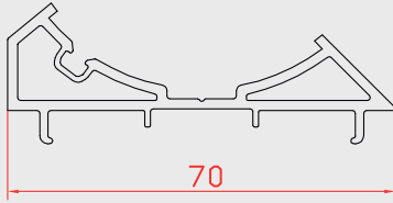
70 mm BORU ADAPTÖRÜ ( Corner Adapter )
