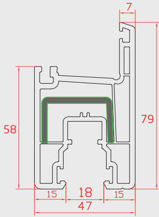
KANAT ( Sliding Sash Profile )
