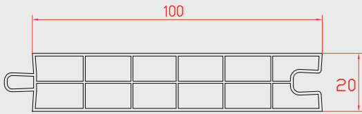
100mm LAMBİRİ ( Two Chamber Panel Profile )
