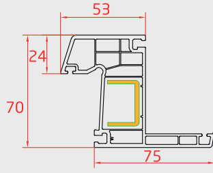
PERVAZLI KASA (Case Profile With Frame)
