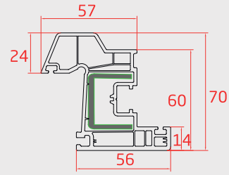
DAMLALIKLI KANAT (Self Drainage Sash Profile)
